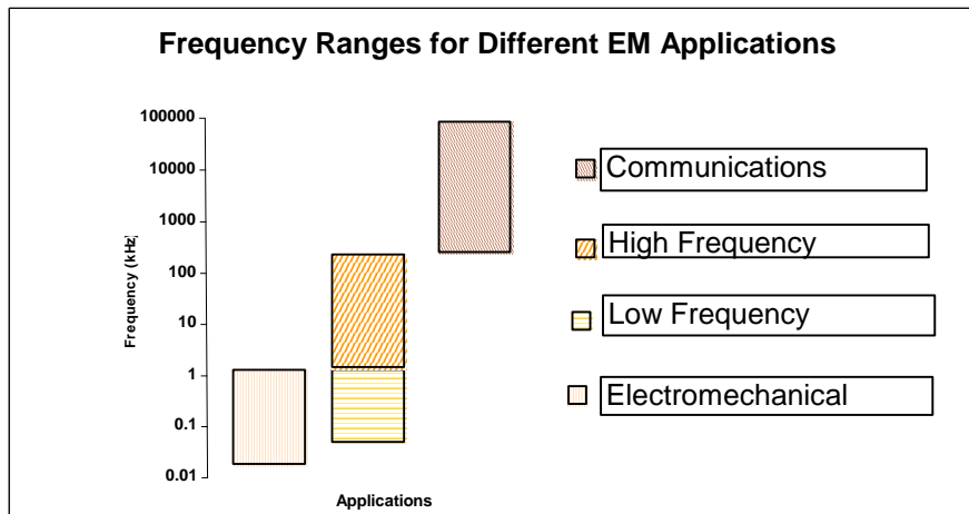
Figure 1 Frequency ranges for electromagnetic applications
