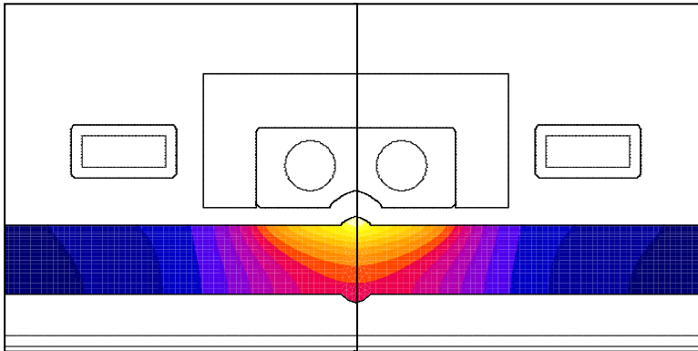
Figure 2. Final temperature distribution for the weld seam stress relieving process using the same coil as for weld seam annealing
