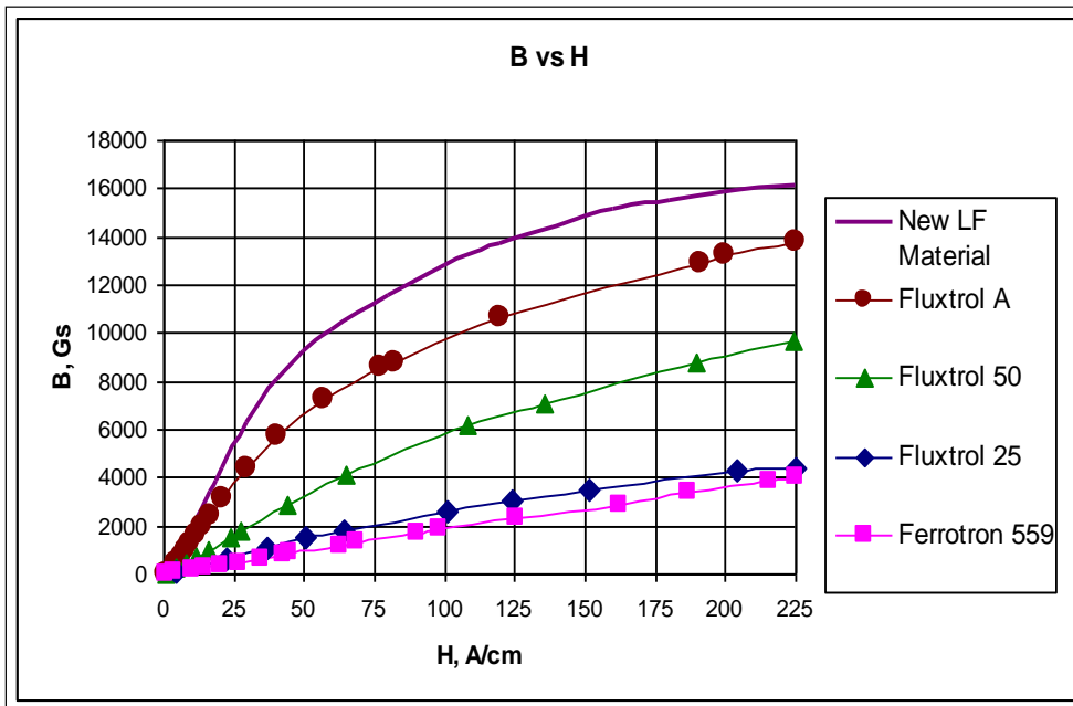
Figure 5. Magnetization curves for MDM's manufactured by Fluxtrol Manufacturing, Inc.
