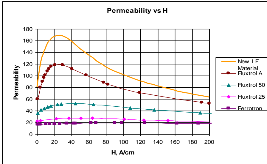
Figure 6. Permeabilities of MDM's manufactured by Fluxtrol Manufacturing, Inc.
