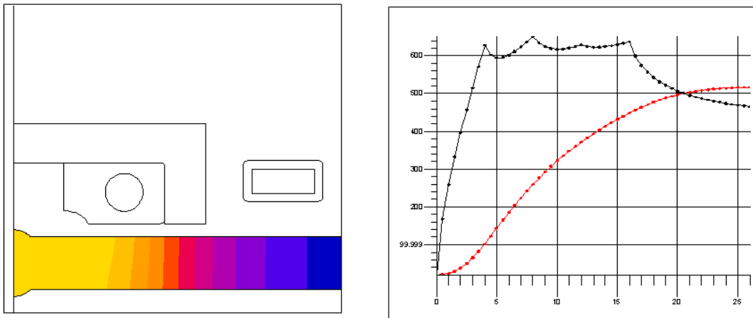
Figure 4. Final temperature distribution and inner and outer weld bead temperature evolution for the optimized coil and process
