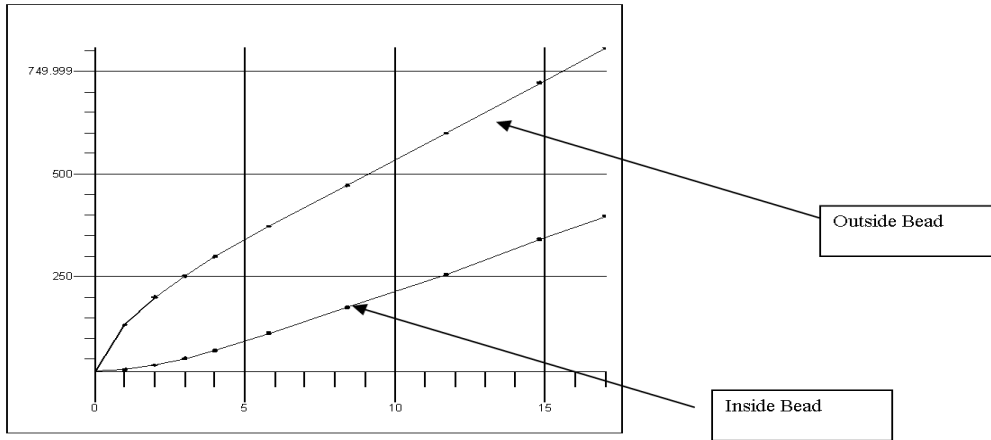
Figure 3. Inner and outer weld bead temperature evolution for the existing stress relieving process
